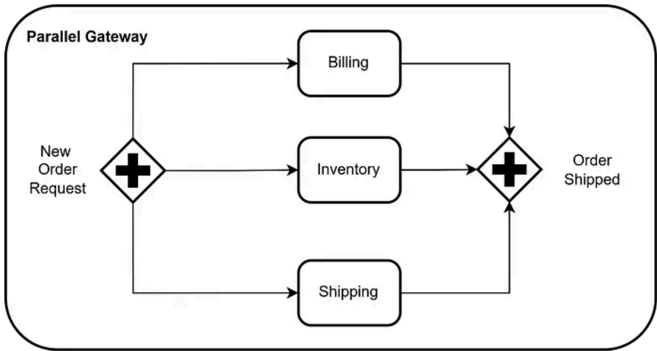
Parallel Gateway
