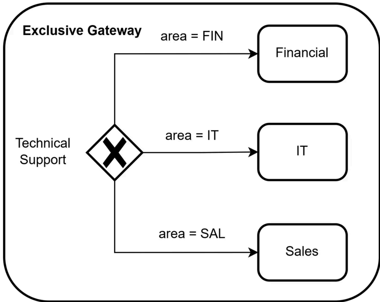
Exclusive Gateway
